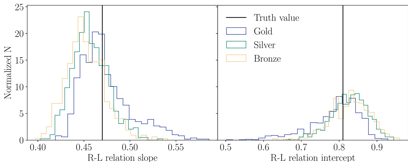
Figure B1. Best-fitting R-L relation slopes ( \frac{\log_{10}(\text{days})}{\log_{10}(\text{erg s}^{-1})} ) and intercepts [ \log_{10}(\text{days}) ] computed using a subsample of sources from each cut group, with corrections for each based on the average offset shown in Table 2. We can see that the biases seen in Fig. 12 are greatly reduced. This indicates that using these simulations to account for biases can be effective.
